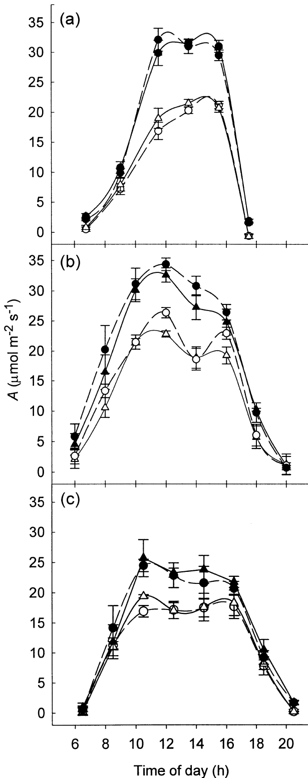
Figure 1. Diurnal time course of the rate of leaf CO 2 uptake ( A ) in Lolium perenne grown at 360 (○, △) and 600 mmol mol -1 (●, ▲) with two N fertilization treatments of 14 (△, ▲) and 56 (○, ●) g N m -2 year -1 . Plants were measured on (a) 18 October 1995; (b) 30 July 1997; and (c) 9 May 2002. Meteorological data describing the dates of measurement is given in Table 1.
