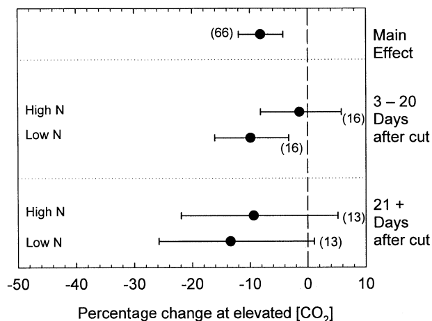
Figure 7. The percentage change of J_{\max} with growth at elevated [\text{CO}_2] . Sample sizes ( n ) for analyses are shown in parenthesis. The mean effect sizes ( r ) surrounded by 95% confidence intervals are shown.
