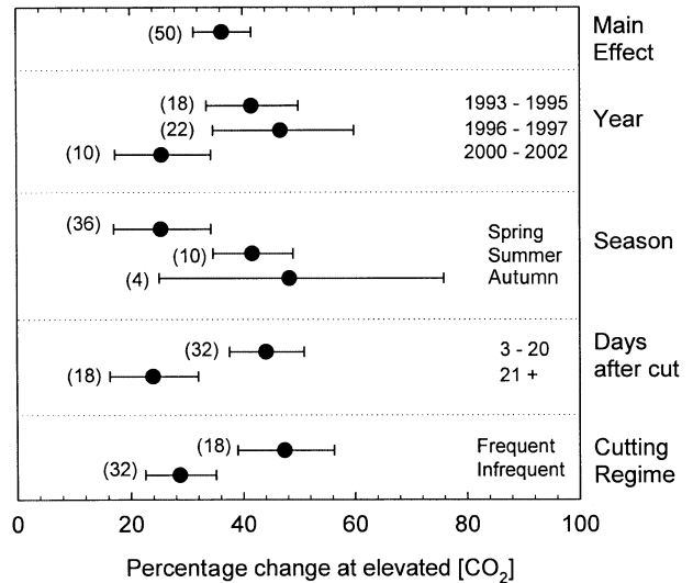
Figure 2. The percentage change of daily integrated carbon assimilation with growth at elevated [CO 2 ]. Sample sizes ( n ) for each categorical treatment are given in parenthesis. The mean effect sizes ( r ) surrounded by 95% confidence intervals are shown.
