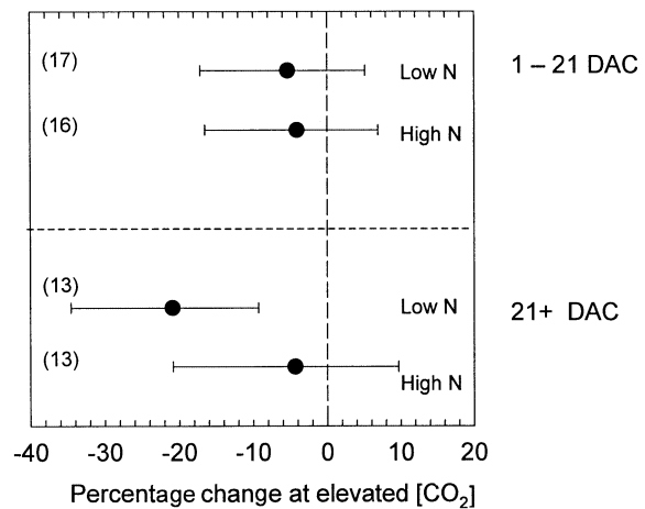
Figure 8. The percentage change in the V_{c,\max}/J_{\max} ratio with growth at elevated [\text{CO}_2] . Sample sizes ( n ) for analyses are shown in parenthesis. The mean effect sizes ( r ) surrounded by 95% confidence intervals are shown.
