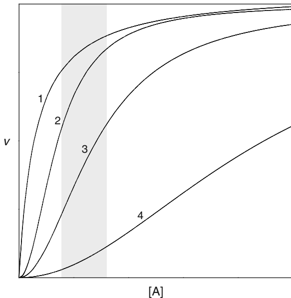
Fig. 4.7 Change in velocity ( v ) with substrate concentration ( [A] ) for an enzyme with normal binding (plot 1) and positive cooperative binding (plot 3) in the presence of an allosteric activator (plot 2) and an allosteric inhibitor (plot 4). The gray area indicates a hypothetical physiological range for this enzyme
