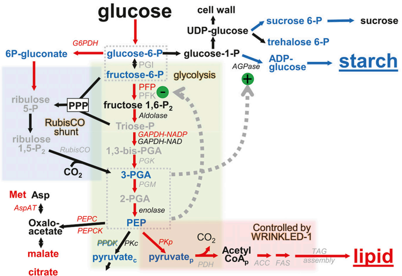
Figure 7. Simplified conceptual model for the central metabolism of oilseed rape and the regulation of carbon partitioning. The network shown represents the most relevant pathways and includes all measured metabolites with strong correlation to flux into fatty acid synthesis or starch ( P < 2\% ). Nonmeasured metabolites are added to complete pathways and are shown in gray. All color-coded fluxes, enzymes, and metabolites have opposite signs in correlation coefficients for lipid and starch, respectively. Red color indicates positive correlation to lipid and negative correlation to starch, being at least in one case highly significant ( P < 2\% ). ACC, Acetyl-coenzyme A carboxylase; FAS, fatty acid synthesis; G6PDH, Glc-6-P dehydrogenase; GAPDH, glyceraldehyde 3-phosphate dehydrogenase; HK-Glc, hexokinase; PDH, pyruvate dehydrogenase; PEPCK, phosphoenolpyruvate carboxykinase; PGI, phosphoglucose isomerase; PGK, phosphoglycerate kinase; PGM, phosphoglycerate mutase; PPK, pyrophosphate:pyruvate dikinase; PPP, pentose phosphate pathway.
