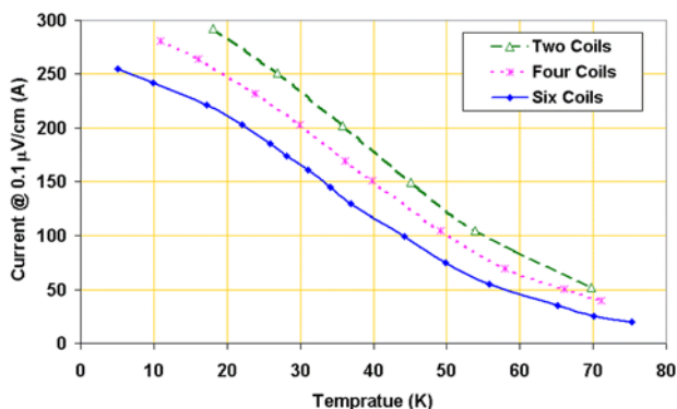
Figure 6: A summary of the temperature dependence of the current in two, four and six coils in the magnetic mirror model. In each case voltage appears on the coil is closest to the pole tip. Note that the magnetic field is approximately three times as great for six coils as it is for four coils.
