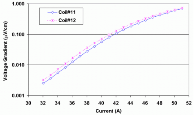
Figure 4: Typical voltage gradient vs. current curves for a pair of coils operated in series in liquid nitrogen bath.
