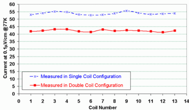
Figure 3: The current at an average voltage gradient of 0.1 \mu\text{V}/\text{cm} ( 10 \mu\text{V}/\text{meter} ) over the total length of the coils measured at 77 \text{ K} for the first thirteen pancake coils powered individually and in pairs.
