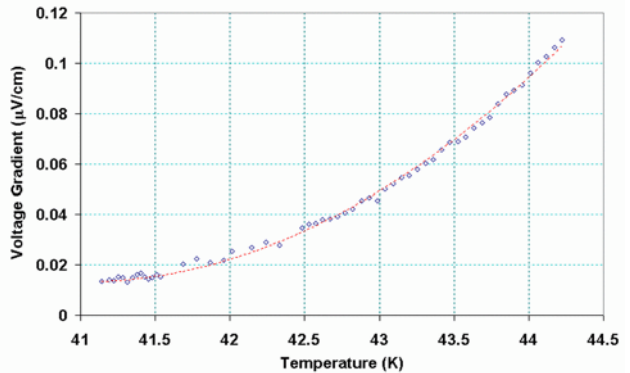
Figure 5: A plot of the voltage gradient as a function of temperature for the magnetic mirror model at a constant current of 100 \text{ A} . The temperature at which the gradient is 0.1 \mu\text{V}/\text{cm} ( 10 \mu\text{V}/\text{meter} ) is seen to be 44.1 \text{ K} .
