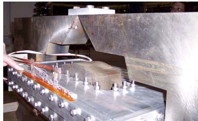
Figure 2: Coils in their bolted support structure, with the pole iron (in the middle, inside the structure), magnetic mirrors (two on the upper side with 45 degree angles on either side of the vertical axis) and iron return yoke.
