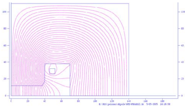
Figure 7: A preliminary magnetic design of an HTS dipole for the Fragment Separator region of RIA.
