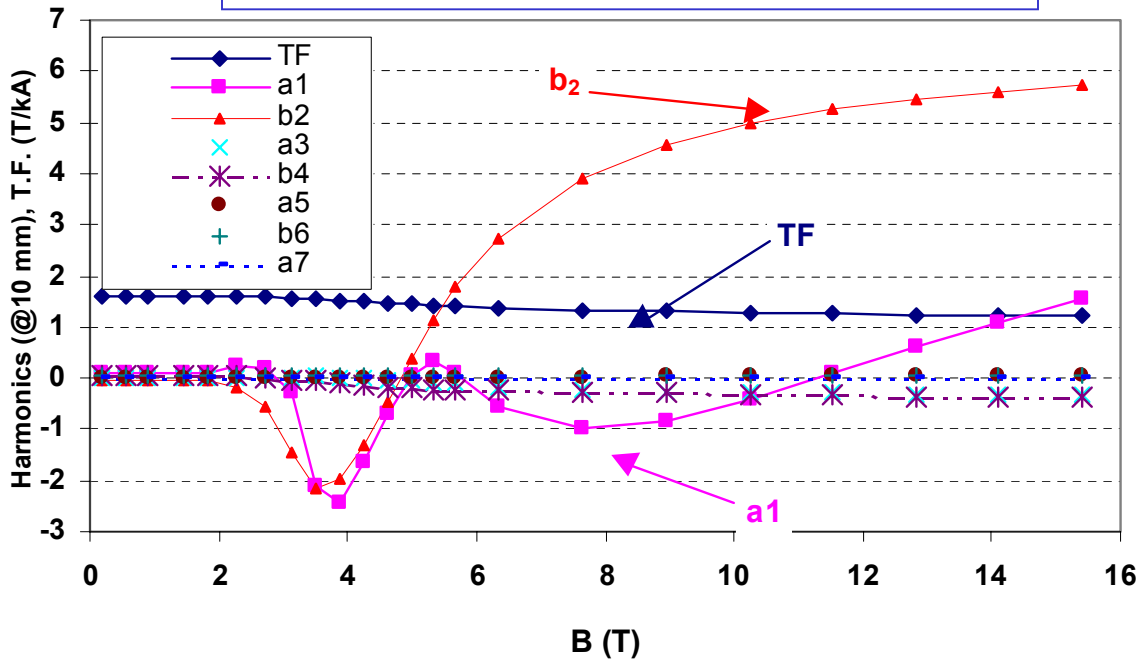
Iron saturation (comparable to cosine theta designs)
