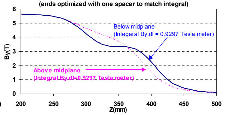
B_y 10 mm above and below midplane on magnet axis (ends optimized with one spacer to match integral)
