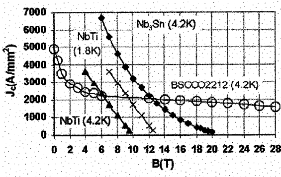
Fig 1: The performance of various superconductors in the year 2000.
