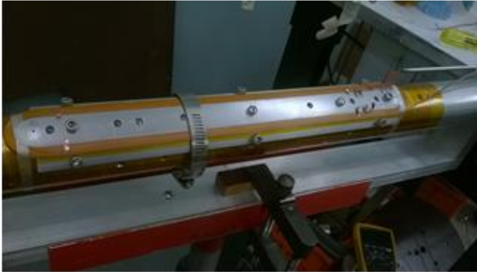
Fig.8. A 45-turn coil wound with ReBCO tape co-wound with Kapton tape.
