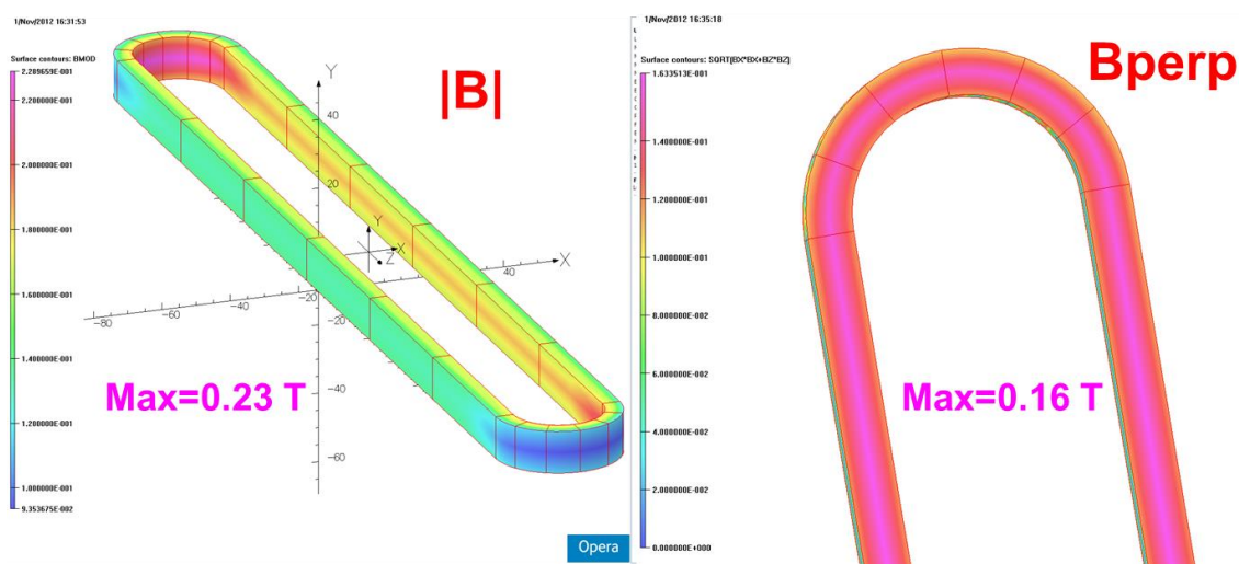
Fig.7. Computed magnitude of the field at 200 A, superimposed on the 20-turn coil on the left and perpendicular component superimposed on the right.
