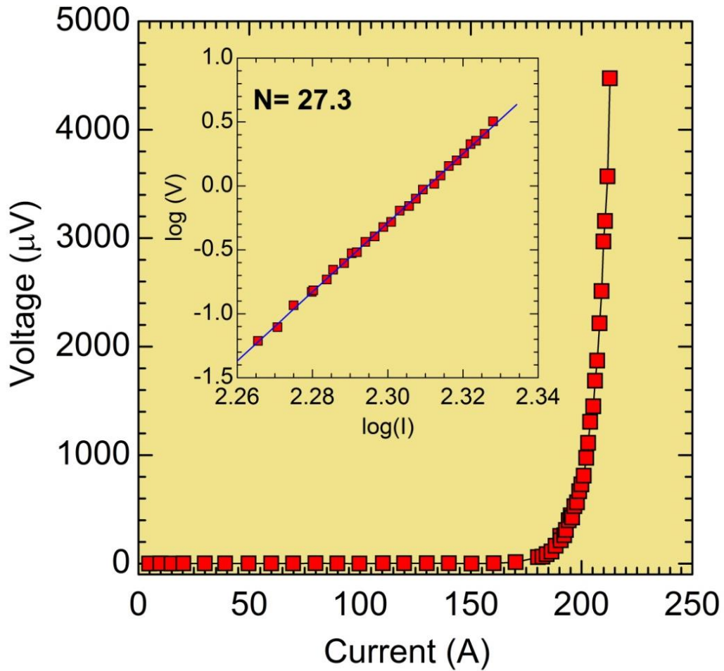
Fig.6. End-to-end coil voltage as a function of current when the 20-turn coil made with the 12 mm tape is tested at 77 K in liquid nitrogen. Insert shows a large n-value, indicating that there was little to no degradation in conductor performance.
