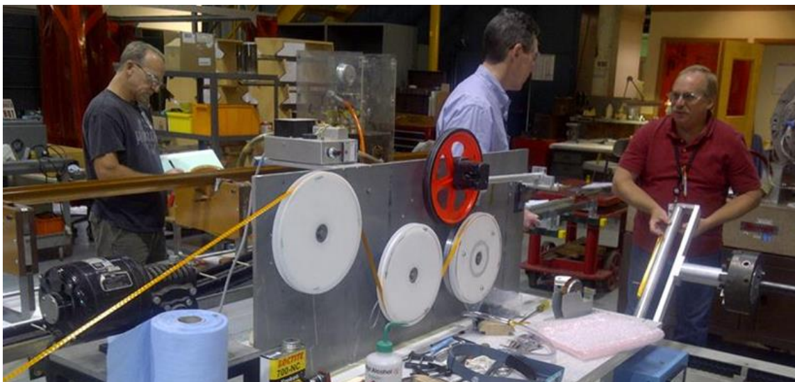
Fig.3. HTS coil being wound on the winding apparatus.
