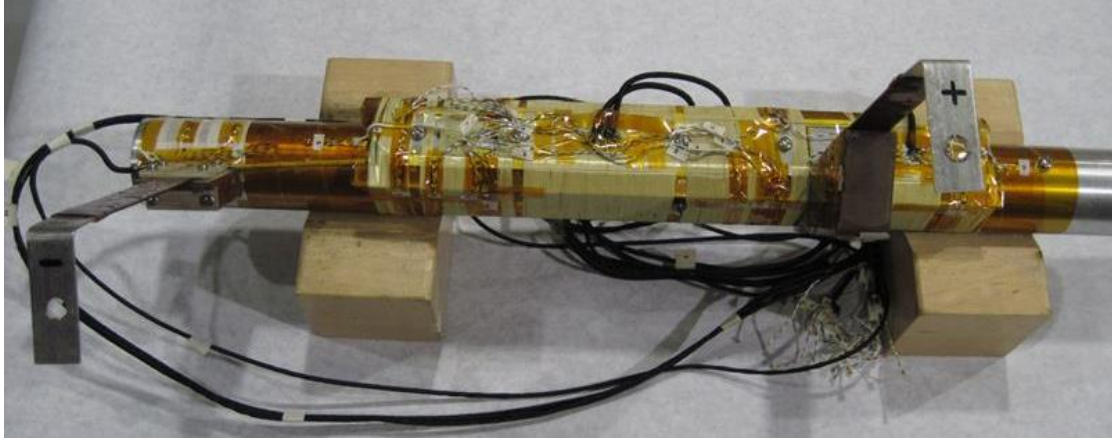
Fig.5. The coil ready for testing at 77 K in liquid nitrogen. The coil has been firmly secured to its mandrel, and current leads and voltage taps are in place.
