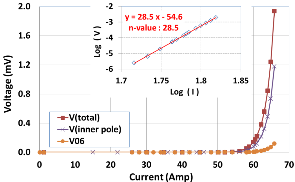
Fig.9. Measured voltage in end-to-end and individual sections as a function of current when the 45-turn coil block made with the 4 mm tape is tested at 77 K in liquid nitrogen. Insert shows a large n-value, indicating that there was little to no degradation in conductor performance.
