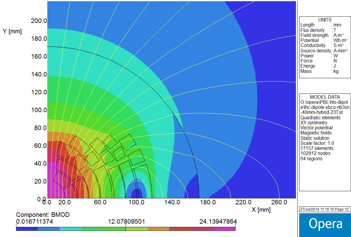
Fig.2. Conceptual magnetic design of a 23.4 T, 40 mm aperture hybrid dipole.
