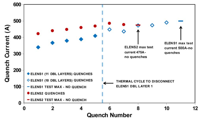
Fig. 3. Plot of quench performance for both main solenoids. Before the indicated thermal cycle, e-Lens1 had 11 double (dbl) layers, and afterward, it had 10 dbl layers and therefore higher operating and maximum test currents than e-Lens2 (473 A instead of 430 A and 500 A instead of 475 A, respectively).
