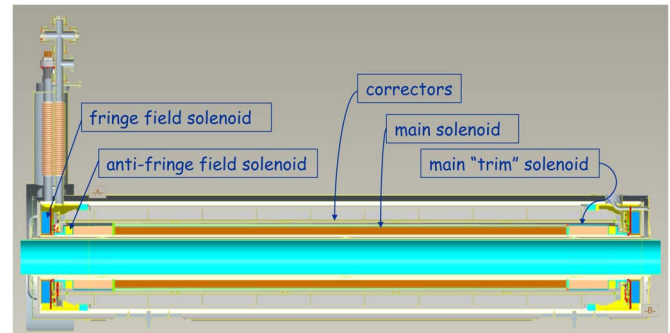
Fig. 1. Cut-away drawing of the e-Lens superconducting magnet system.
