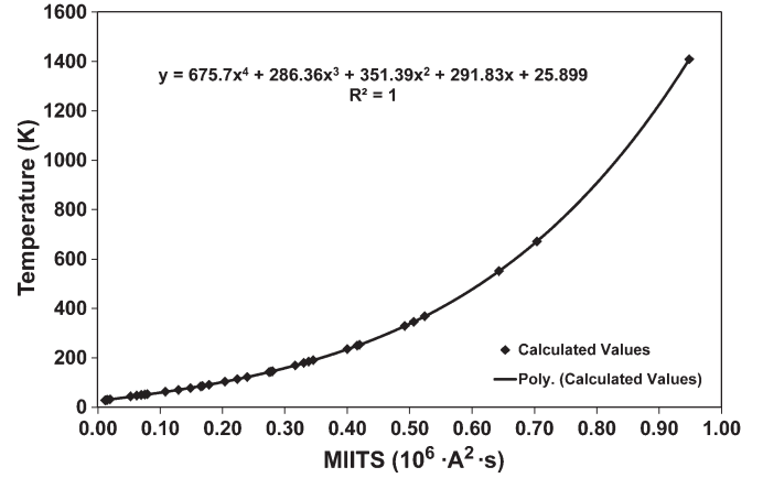
Fig. 2. Plot of hot spot temperature versus MIITs for main solenoid.
