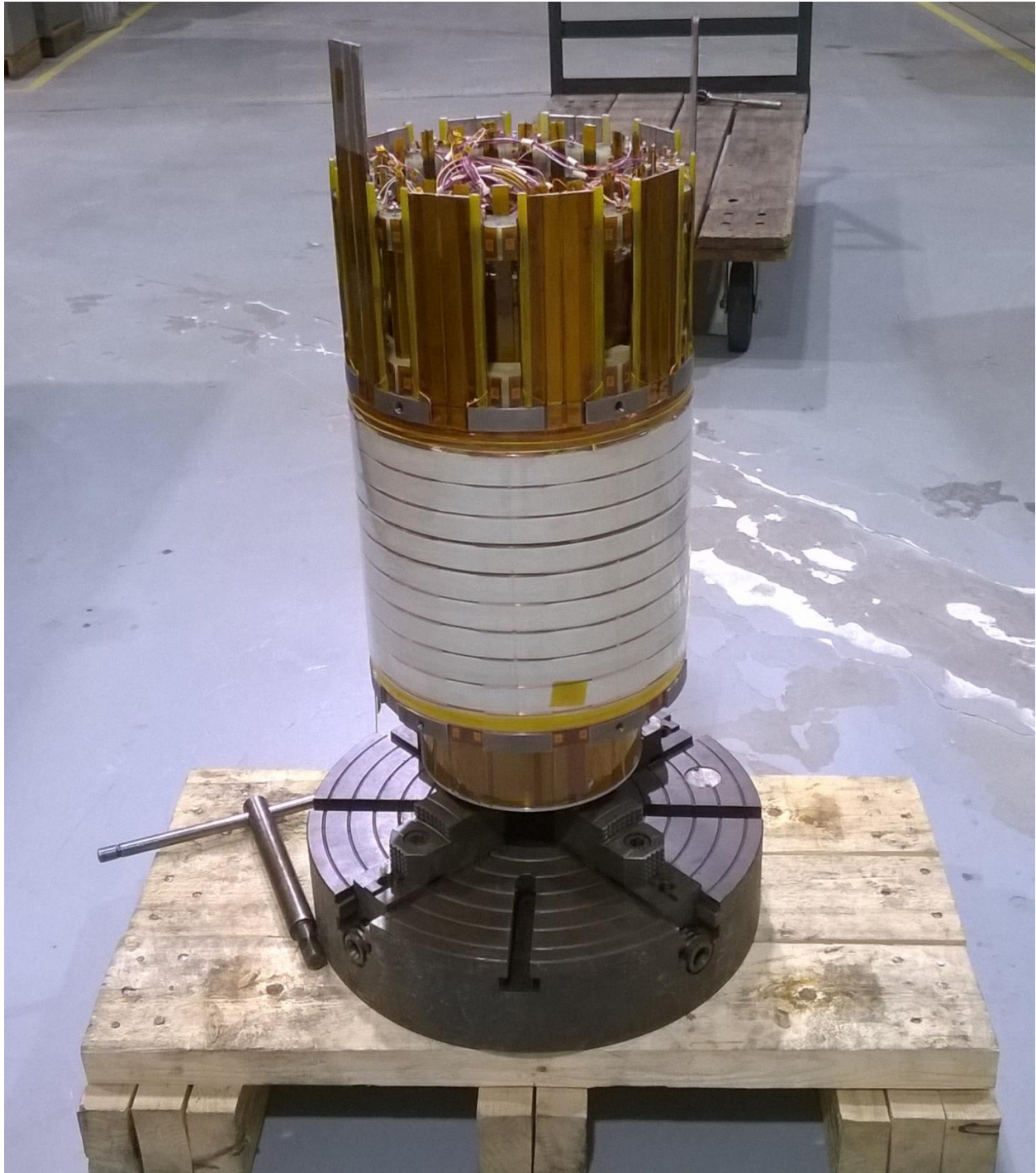
Figure 18: Outer coil being prepared for installation of outer support tube.
