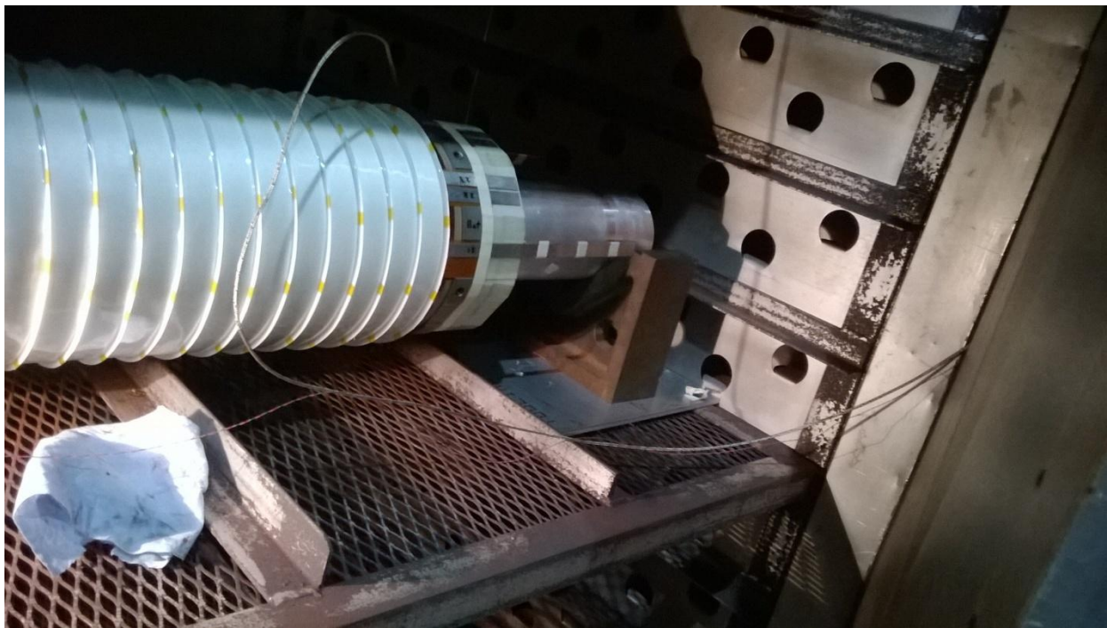
Figure 3: Inner pancake coil assembly inside the oven for curing after fiberglass epoxy tape was wrapped around it.
