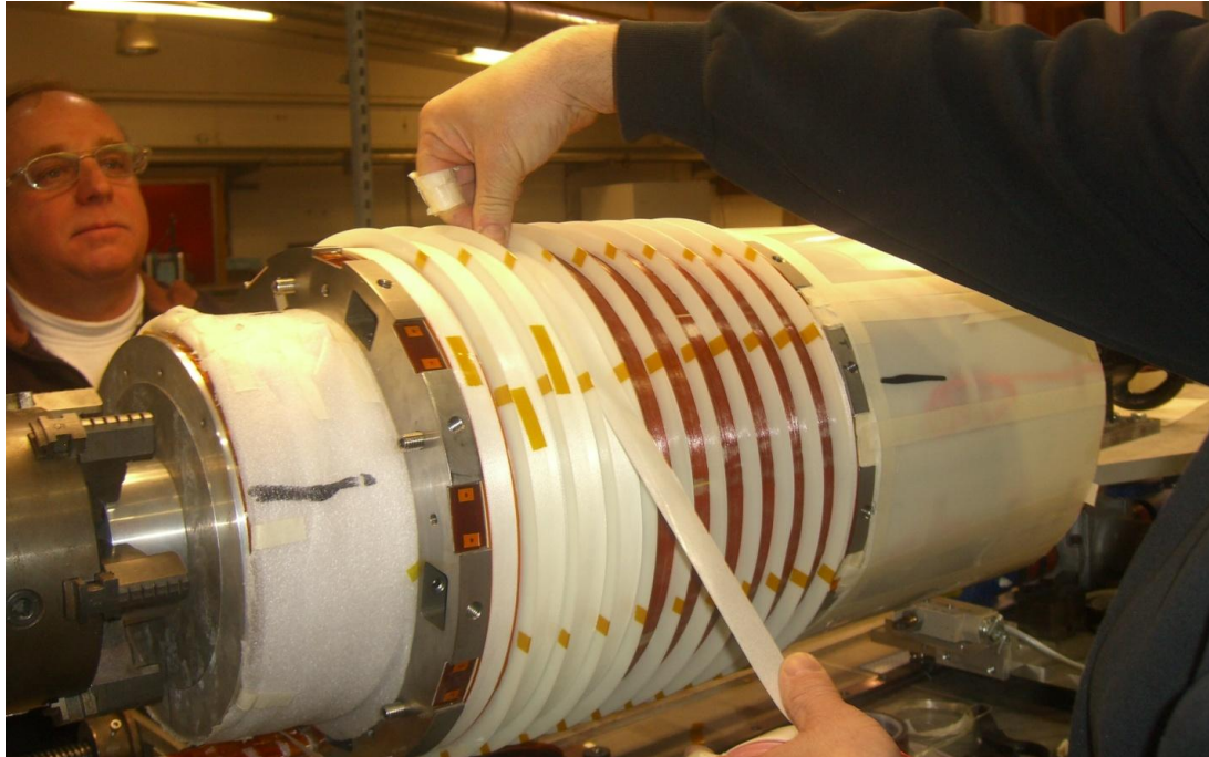
Figure 14: Fiberglass tape is being wrapped over the double pancake of the outer layer before curing.
