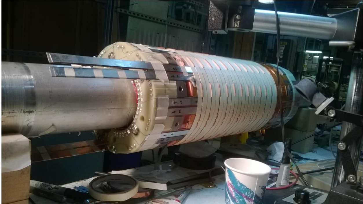
Figure 1: All leads installed, v-taps wires taken out and Nomex filler pieces placed in between and around the leads of the inner layer.
