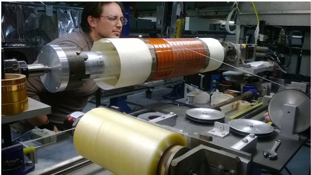
Figure 2: Kevlar string being put over the kapton which covers the inner pancake coil assembly.
