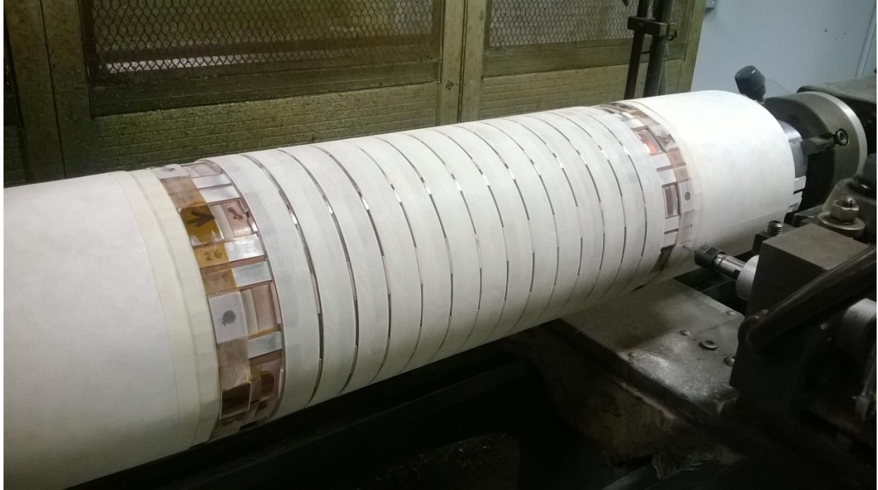
Figure 5: Inner pancake coil assembly after outer surface machined to required diameter.
