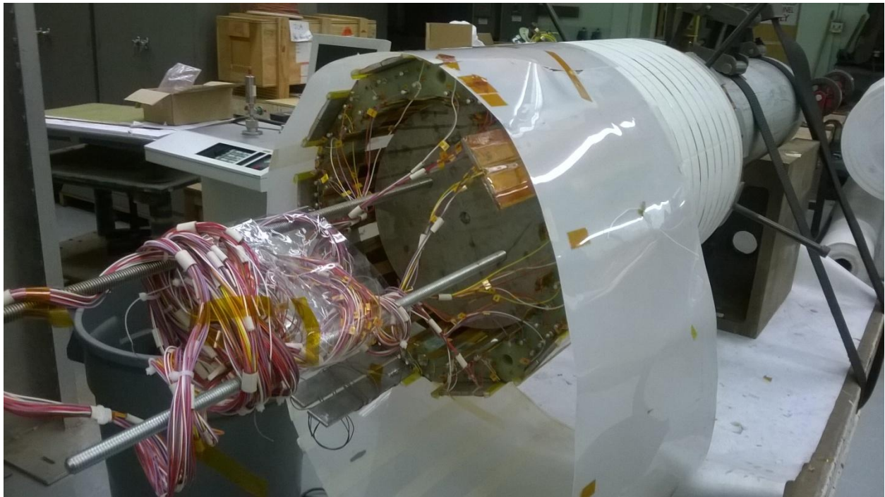
Figure 11: A large number of instrumentation wires installed on the outer coil assembly to monitor onset of any resistive voltage across any pancake or joint during the test. The complete set of instrumentation also includes a number of temperature sensors.
