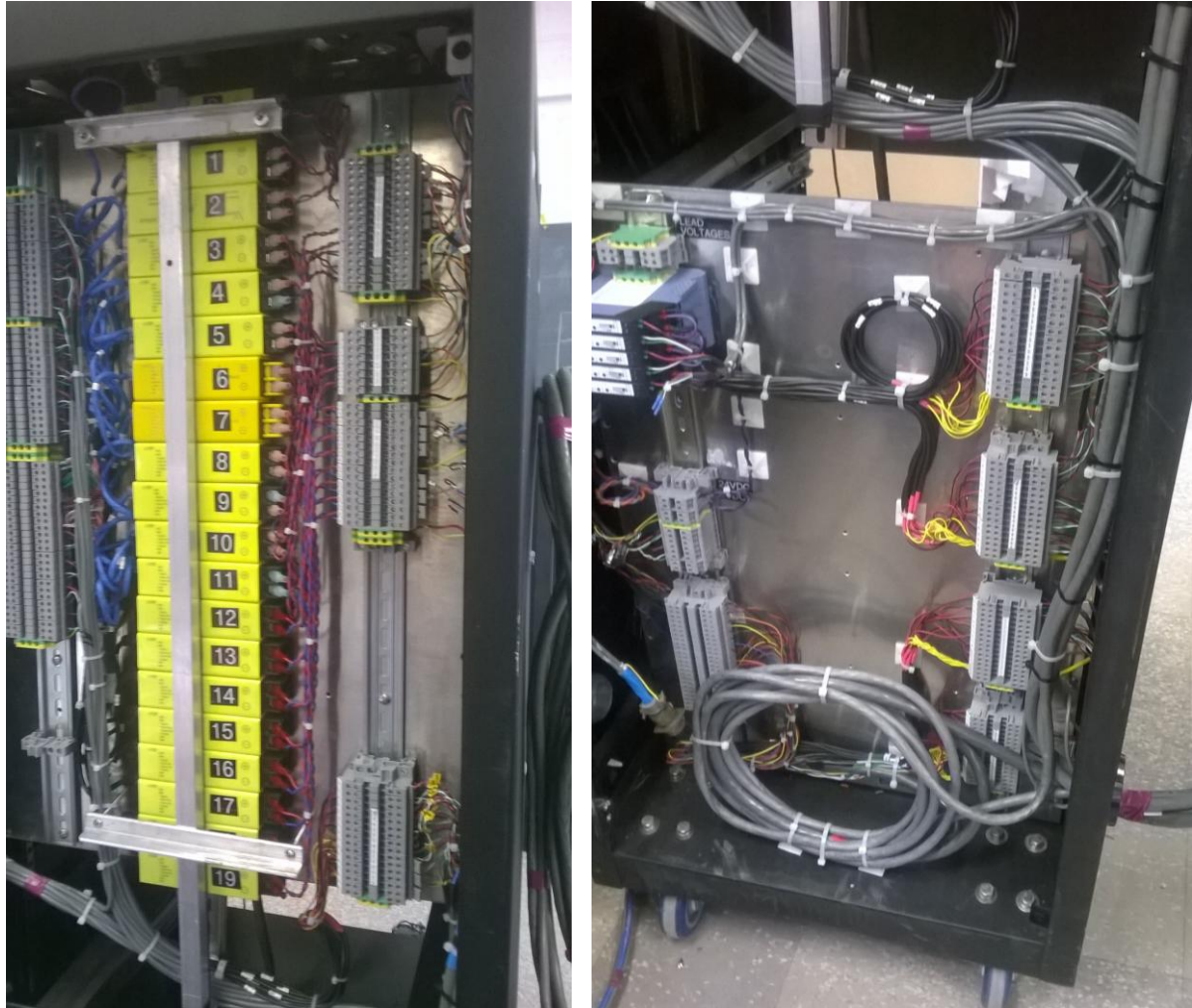
Figure 22: Expanded quench detection and protection system with high voltage isolators.
