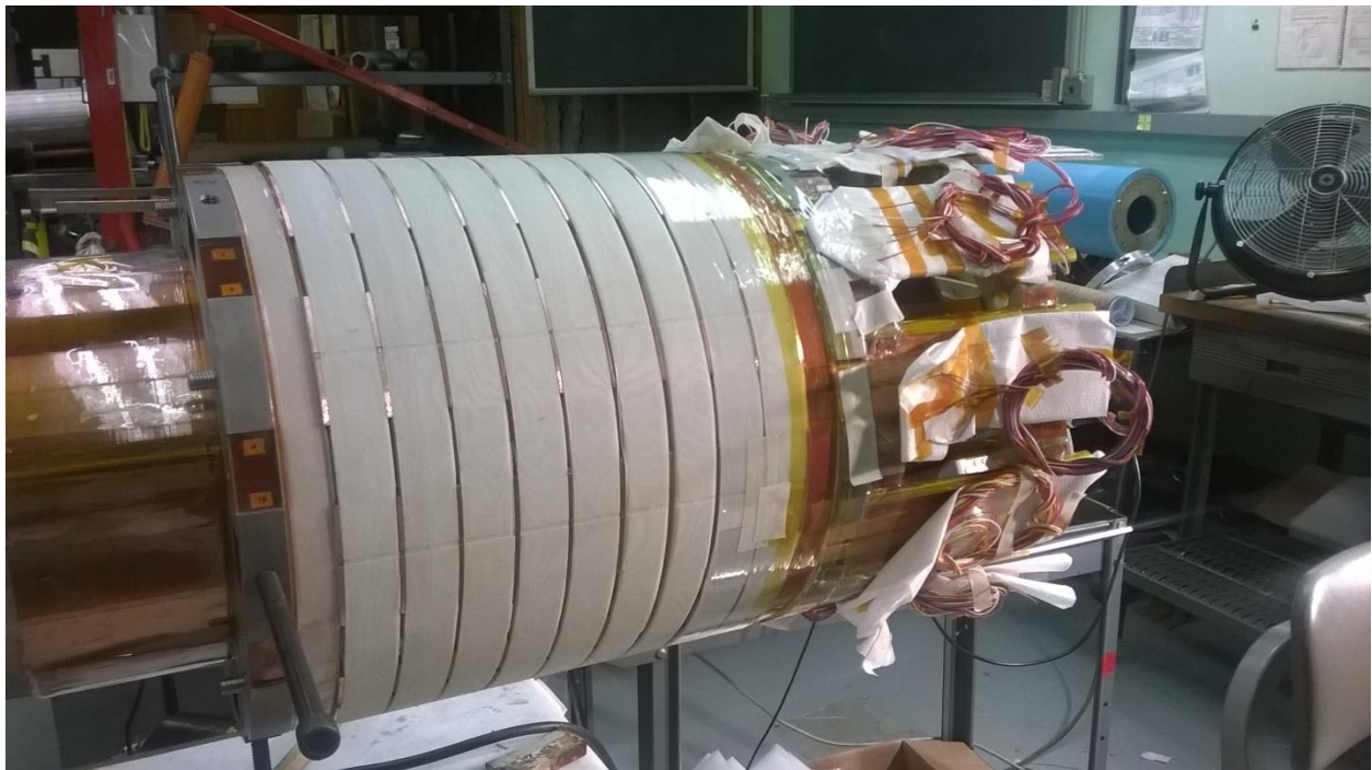
Figure 17: Full view of the outer coil after machining with instrumentation wires.
