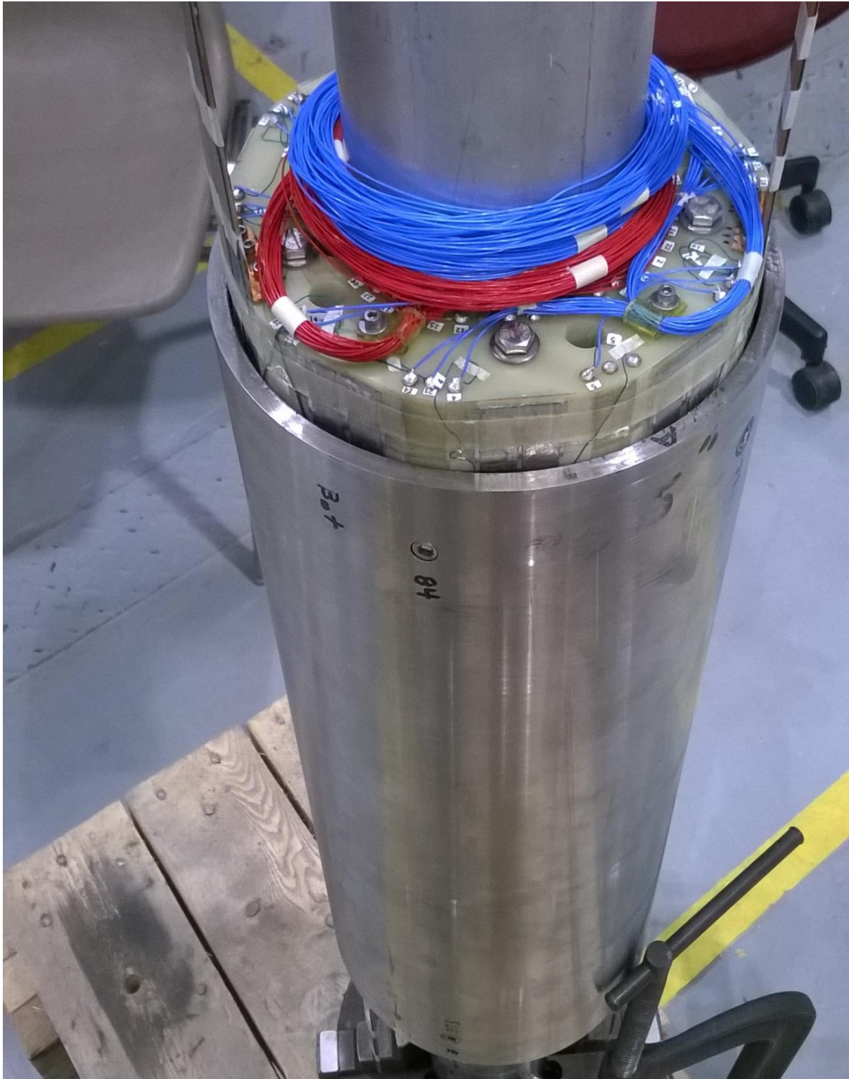
Figure 7: Complete inner pancake coil with outer stainless steel support tube structure installed over the coil. One can also see instrumentation wires (red connected to those coming from inside and blue from outside).
