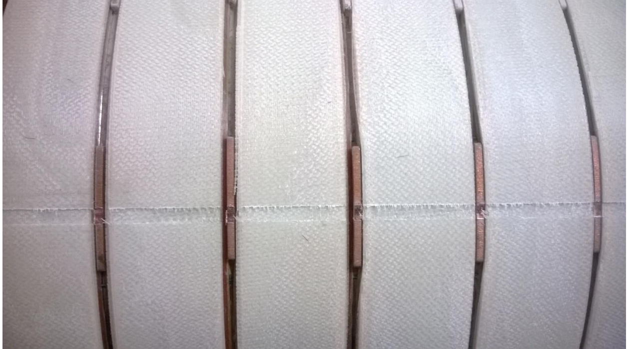
Figure 6: Inner pancake coil assembly with grooves cut for helium flow for uniform cooling. One can also see copper discs between each pair of double pancakes to provide more uniform radial cooling
