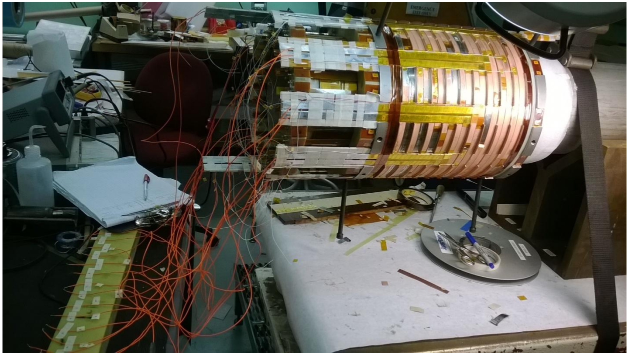
Figure 8: Preparation for high-pot test for outer pancake coil assembly.
