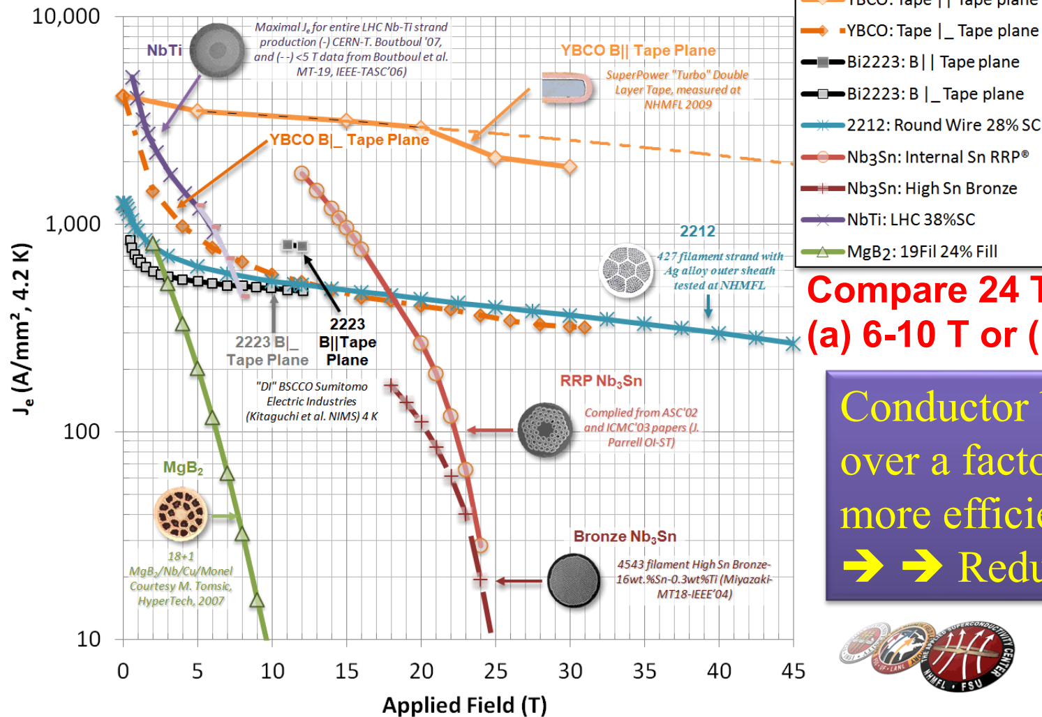
Current Density Across Entire Cross-Section
