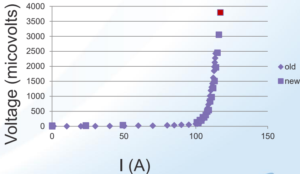
bottom coil
