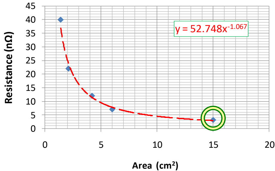
Simulation of splice joint within coil
