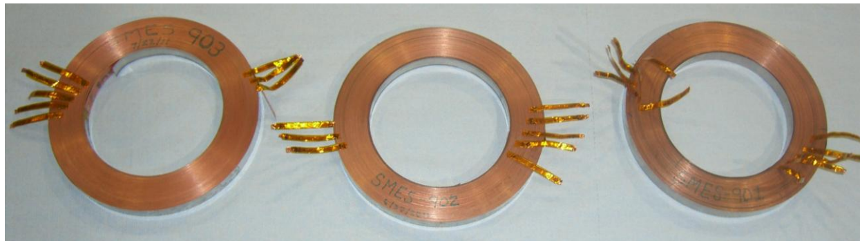
Fig. 5: Three test coils wound with ~12 mm 2G HTS received from SuperPower.
