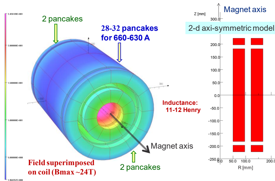
Fig. 1: 3-d (left) and axis-symmetric 2-d model (right) of the current design of the 2.5 MJ demo device.
