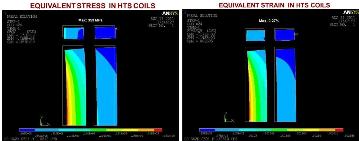
Fig. 4: Computed stress and strain in the HTS coils based on a simplified ANSYS model.
