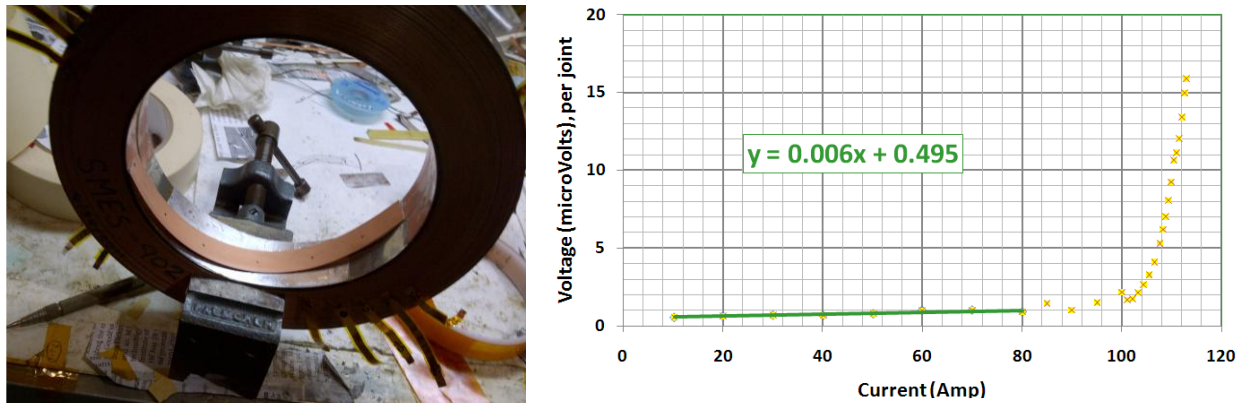
Fig. 7: Geometry of the new coil-to-coil diagonal joint on left and 77 K test results showing ~6 nano-ohms measured resistance per joint on right.
