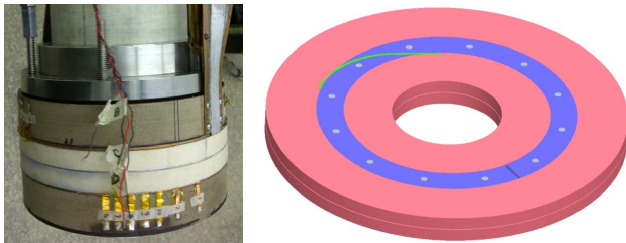
Fig. 6: Two of three test coils shown in Fig. 5 being prepared for a double pancake coil test (left). These coils will continue to be wound after the test with an internal support structure (right).
