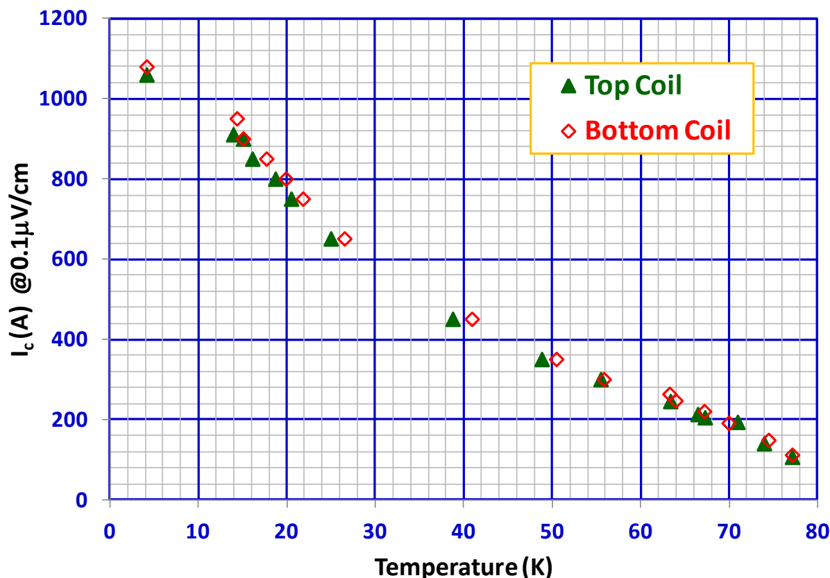
Fig. 11: A comprehensive summary of the test results. The coils were tested well above the design current of ~660 A. The tests below 60 K were carried out with helium and above 60 K with nitrogen.
