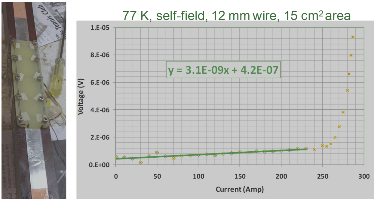
Fig. 8: Geometry of the internal splice joint based on techniques used in magnet division over a decade on left and 77 K test results showing ~3.1 nano-ohms measured resistance per joint on right.
