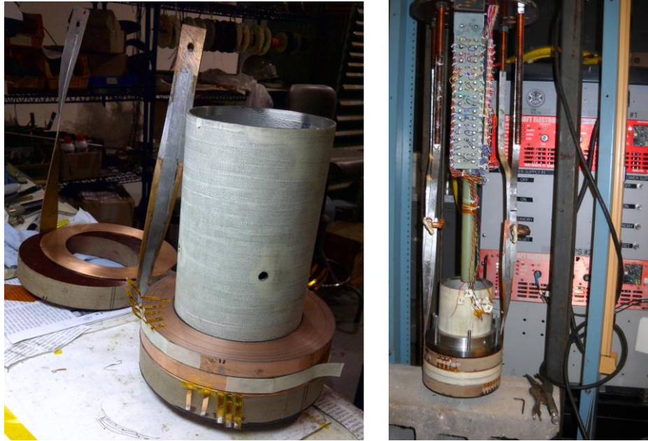
Fig. 9: Coils being prepared for test on left and installed on the top-hat to test them to \sim 1000 A on right.
