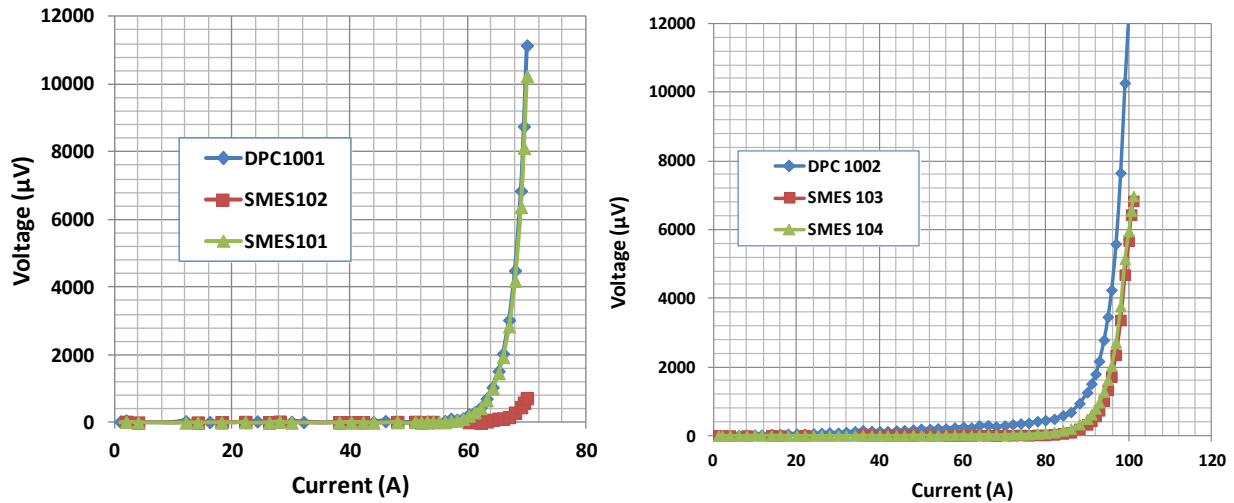
Fig. 5: Voltage across the individual pancakes (SMES101 thru SMES104) and double pancakes (DPC1001 and DPC1002) as a function of current in first four pancakes tested in liquid nitrogen.
