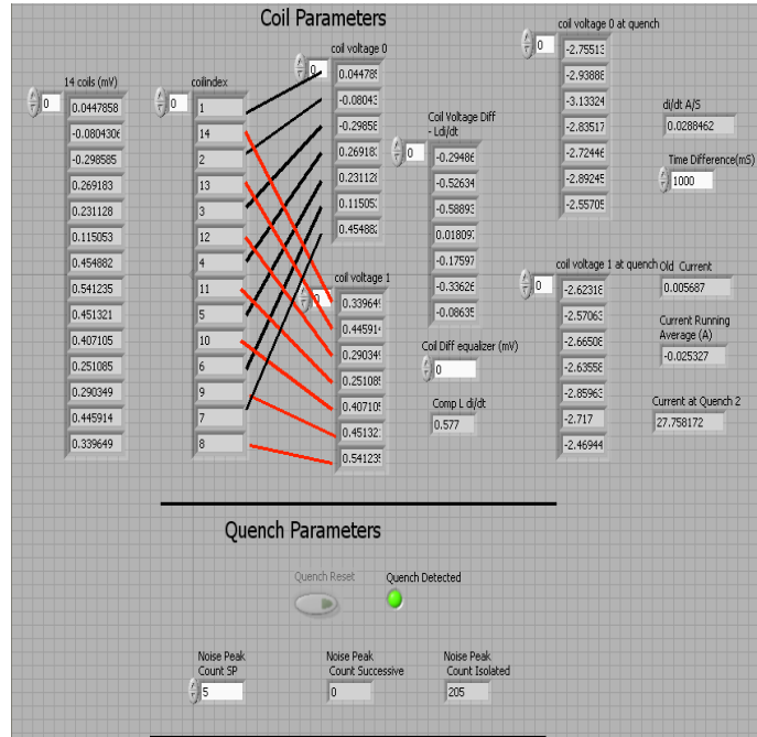
Fig. 7: Hardware (left) and screenshot of Labview software (right) for the quench protection system of SMES.
