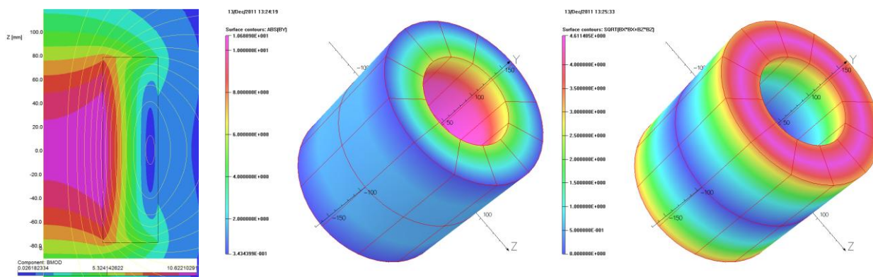
Fig. 1: 2-d axis-symmetric and 3-d magnetic model of the SMES coil to be tested in Q6. Parallel (maximum 10.7 T at SMES coil design current) and perpendicular (maximum 4.6 T at SMES coil design current) components of the field are shown on the surface of the 3-d model.
