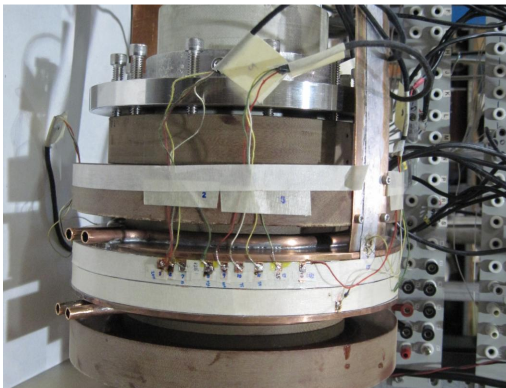
Fig. 3: A double pancake coil in a fixture ready for 77 K test in liquid nitrogen.
