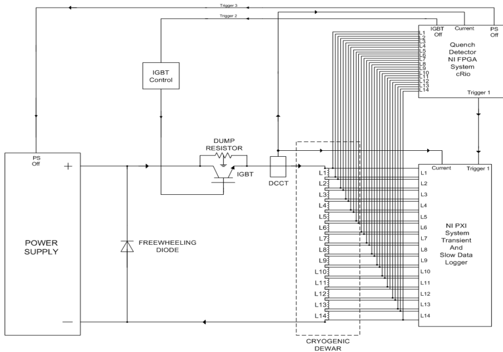
Fig. 6: Schematic of the 14 channel Quench Protection System (QPS).
