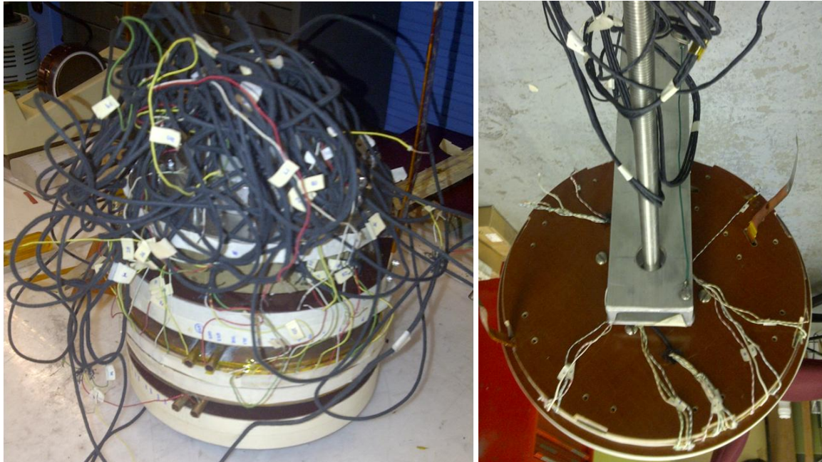
Fig. 3: A double pancake coil for inner layer just after the 77 K test (left) and a simpler single pancake coil test set-up for limited test (right).
