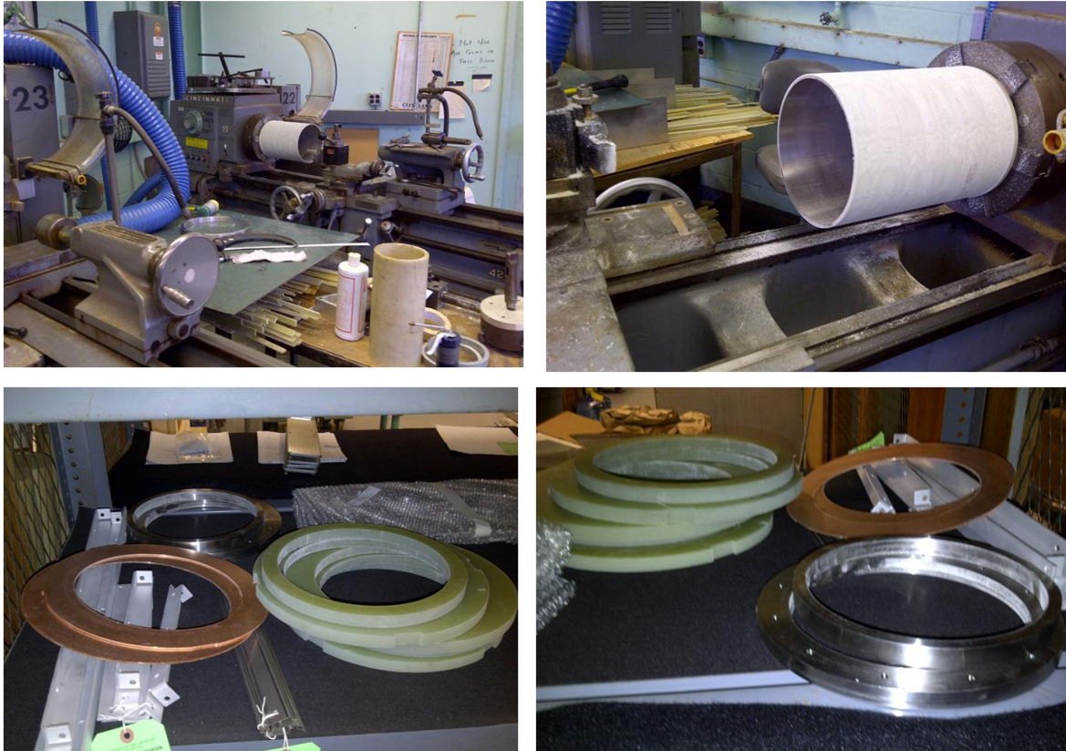
Fig. 4: Parts for making fixture for testing outer double pancake coils at 77 K.
