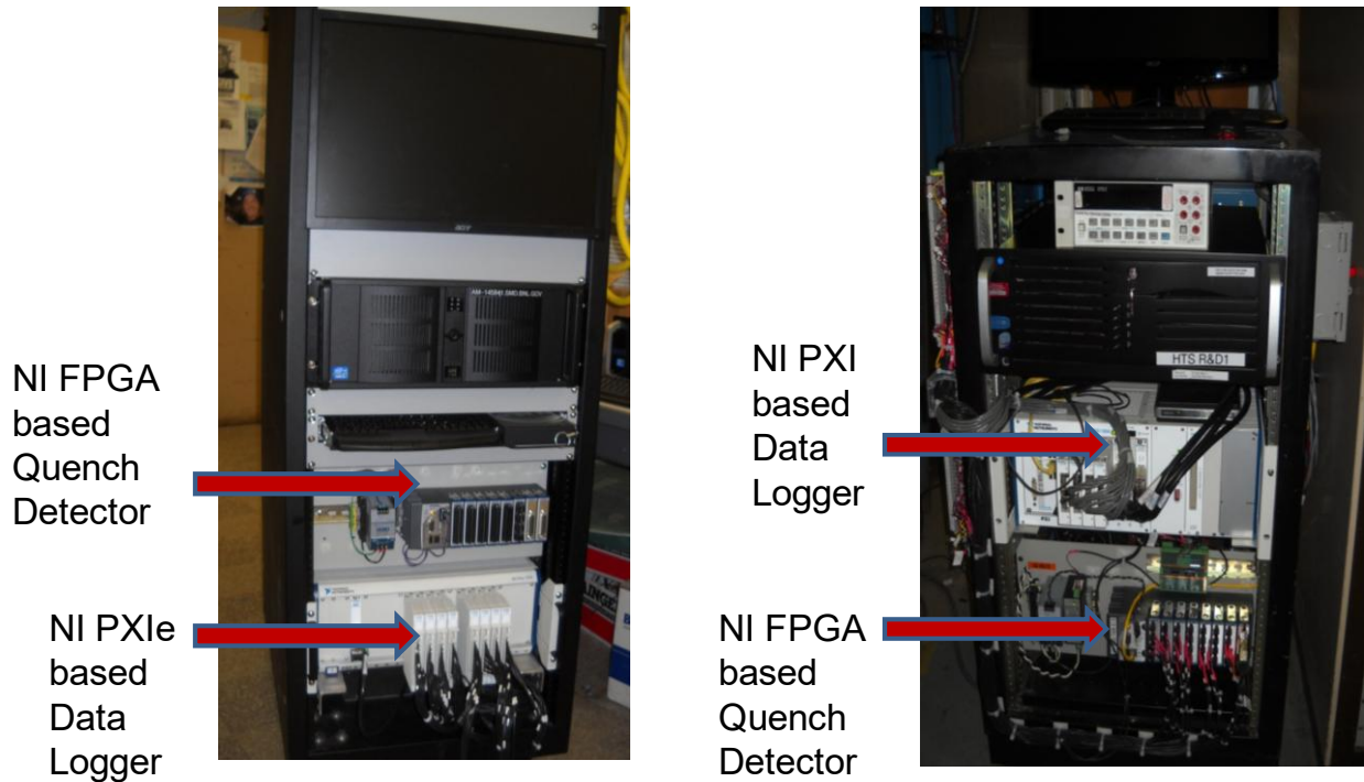
Fig. 2: Control and quench detection system.
