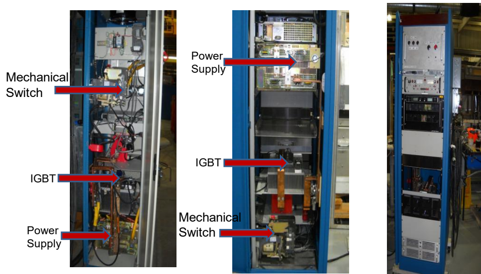
Fig. 1: Views of two power supplies and the energy extraction system. Location of individual component is indicated
