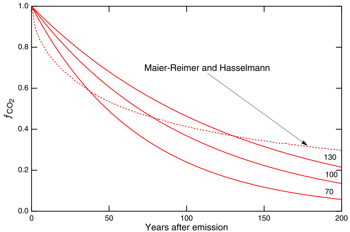
Figure 2. Profiles of fraction of excess CO 2 remaining in atmosphere as function of time subsequent to introduction into atmosphere. Solid curves show exponential decay for indicated mean residence times in years. Dotted curve shows nonexponential decay curve obtained with multi-component box model, as employed in Global Warming Potential estimates by IPCC. 14
