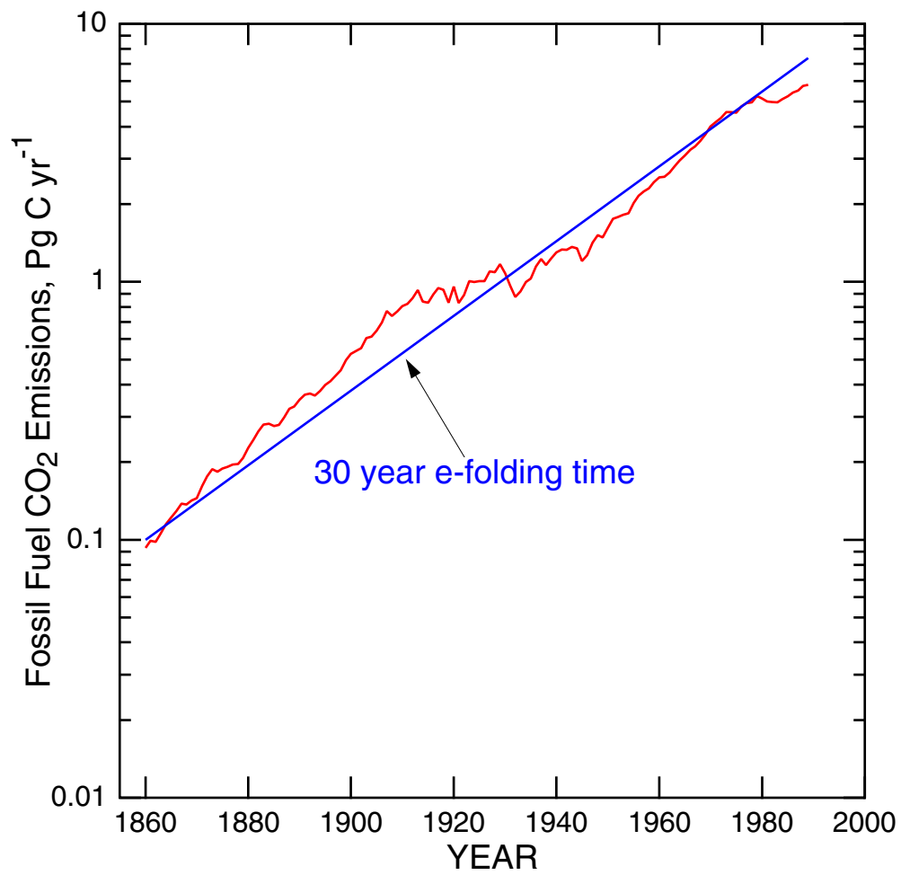
Figure 4. Rate of anthropogenic CO 2 emissions from fossil fuel combustion over the industrial era. 28 Straight line represents exponential growth with 30 year e-folding time.
