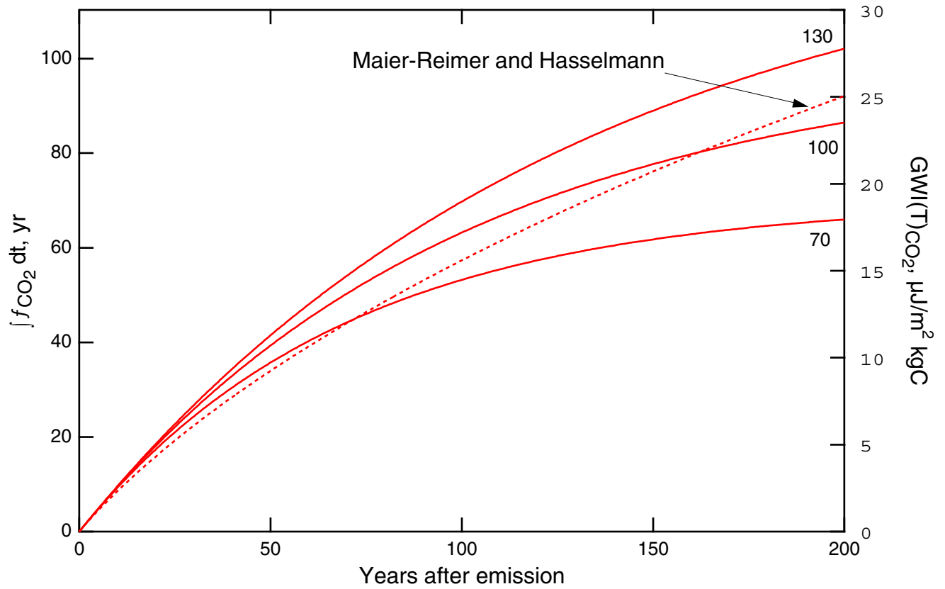
Figure 3. Profiles of the time integral of the fraction of excess \text{CO}_2 remaining in atmosphere as function of time subsequent to introduction into atmosphere. Solid curves shows integral of exponential decay for indicated mean residence times in years. Dotted curve shows integral of nonexponential decay curve obtained with multi-component box model. Right hand axis shows Global Warming Integral evaluated for the instantaneous radiative forcing due to an incremental amount of \text{CO}_2 in the atmosphere a_{\text{CO}_2} = 8.6 \times 10^{-15} \text{ W m}^{-2} \text{ per kg C} .
