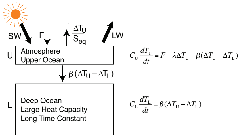
Figure 1. Two-compartment model for Earth's climate system, consisting of upper compartment U with small heat capacity C_U and short time constant for reaching steady state following a perturbation, and lower compartment L with large heat capacity C_L and long time constant for reaching steady state. Thick arrows denote initial shortwave (SW) and longwave (LW) fluxes, and thin arrows denote perturbations: forcing F and resultant heat flows, a change in net top-of-atmosphere irradiance given by the time-dependent forcing minus the time-dependent change in temperature \Delta T_U of the upper compartment upon the equilibrium sensitivity S_{eq} , and a heat flux from the upper compartment to the lower compartment L given by the heat exchange coefficient \beta times the difference in temperature changes between the upper ( \Delta T_U ) and lower ( \Delta T_L ) compartments.
