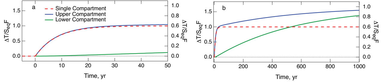
Figure 2. Normalized temperature response of one- (left axis) and two-compartment (right axis) models to step function forcing initiated at time = 0. Equilibrium sensitivity of one-compartment model and transient sensitivity of two-compartment model are 0.4 \text{ K (W m}^{-2}\text{)}^{-1} ( \Delta T_{2x} = 1.5 \text{ K} ); equilibrium sensitivity of two-compartment model is 0.67 \text{ K (W m}^{-2}\text{)}^{-1} ( \Delta T_{2x} = 2.5 \text{ K} ). Heat exchange coefficient in two-compartment model is 1 \text{ W m}^{-2} \text{ K}^{-1} . Time constant of one-compartment model and of upper compartment of two-compartment model is 8 years; time constant of lower compartment is 570 years. Heat capacity of upper compartment and lower compartment are 20 and 340 \text{ W yr m}^{-2} \text{ K}^{-1} , respectively. Vertical axes are scaled by the ratio of the equilibrium sensitivities of the two models.
